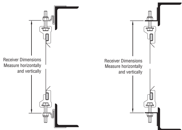
FIG. 1 E-Hook and Receiver
