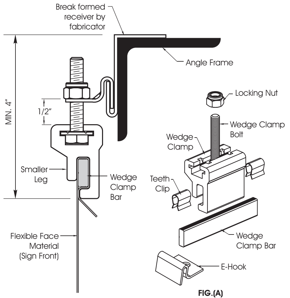
Wedge Clamp Assembly
