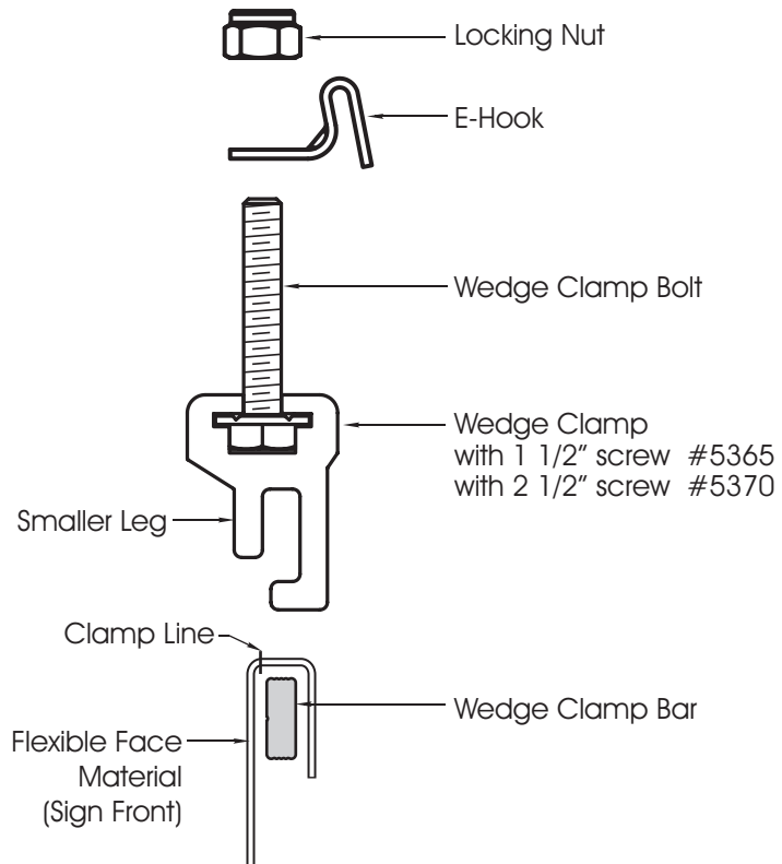
Wedge Clamp Assembly
